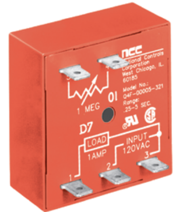
.25 X .032 MALE FAST-ON TERMINALS (7 PL.)
